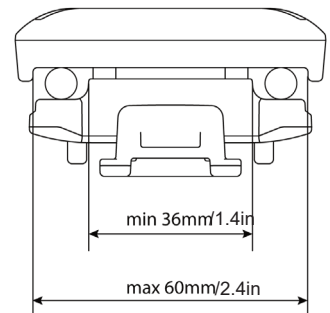
Mounting set for saddle bag (included)
